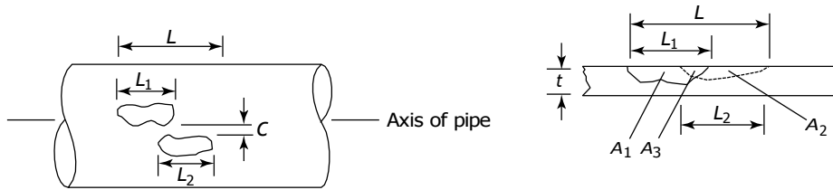
Figure 451.6.2.2-1 Type I Interaction
