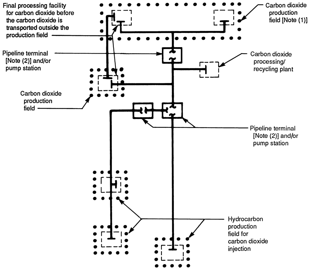
Figure 400.1.1-2 Diagram Showing Scope of ASME B31.4 for Carbon Dioxide Pipeline Systems
