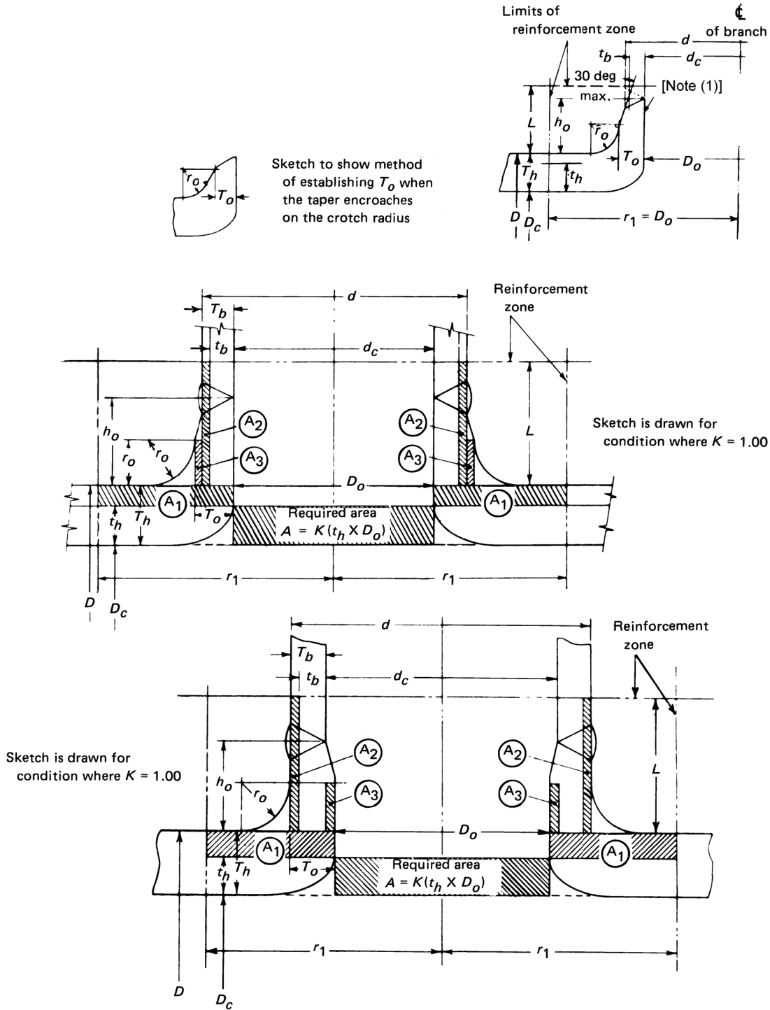
Figure 404.3.3.1-1 Reinforced Extruded Outlets
