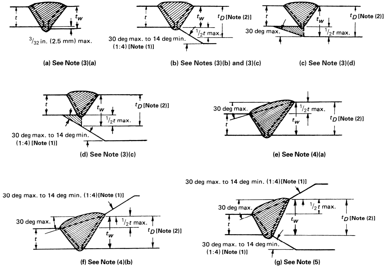
Figure 434.8.6-2 Acceptable Butt Welded Joint Design for Unequal Wall Thicknesses
