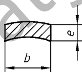
Figure 6 — Bar-shaped test piece for impact strength test
