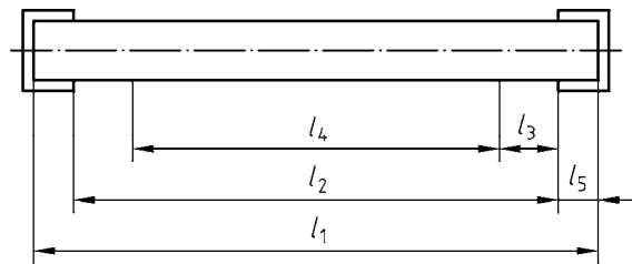
Figure 5 — Test pieces for long-term hydrostatic test
